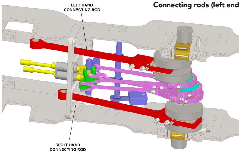
Connecting rods (left and right hand).
