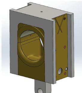
CAD image of Axlebox
